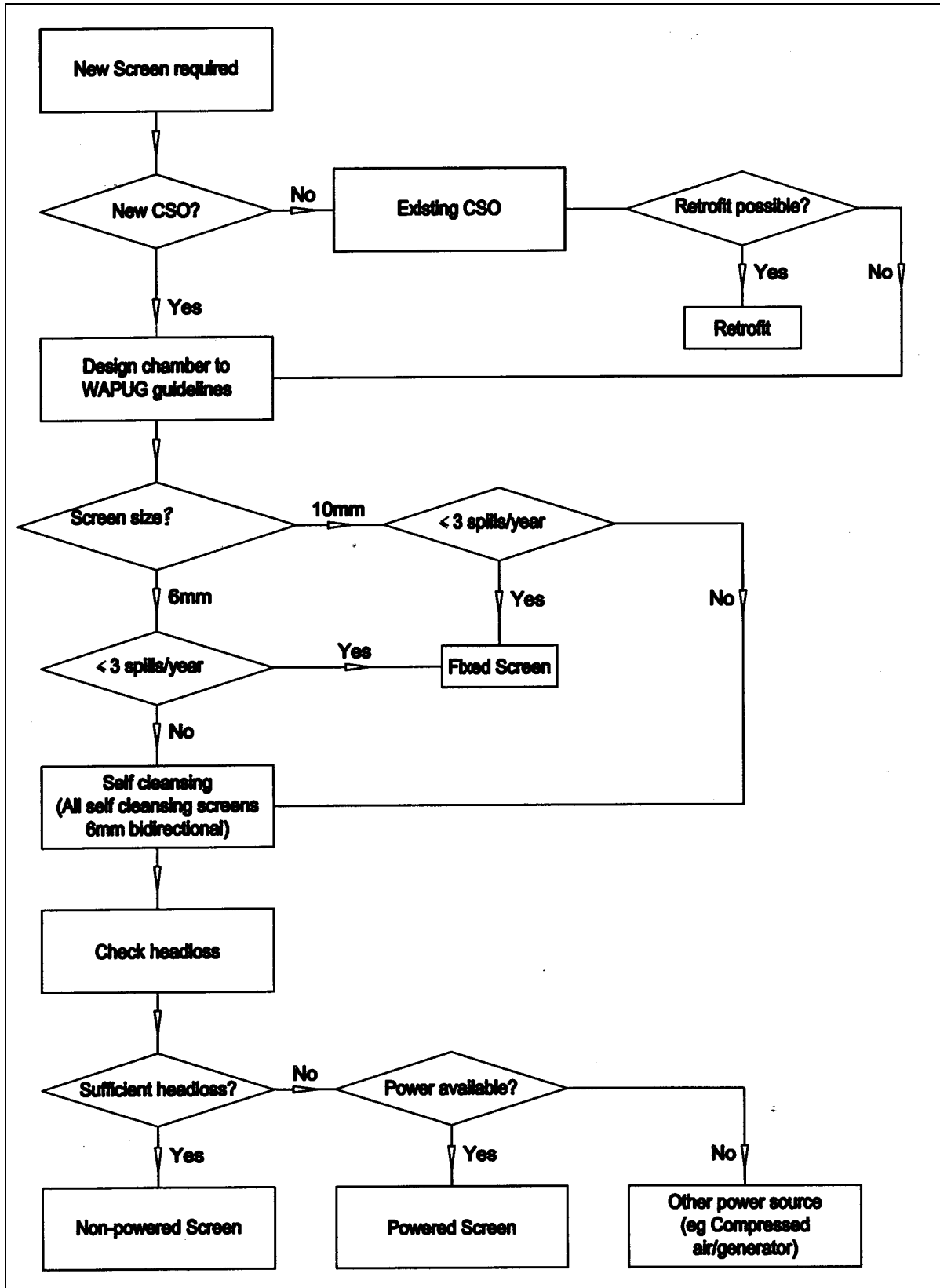
Figure G1 Flowchart for CSO Screen Selection
