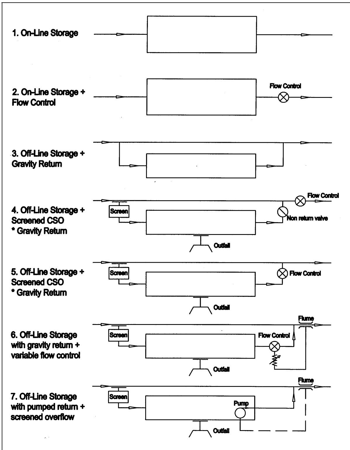
Figure G2 Arrangements for Storage, CSOs and Screens
