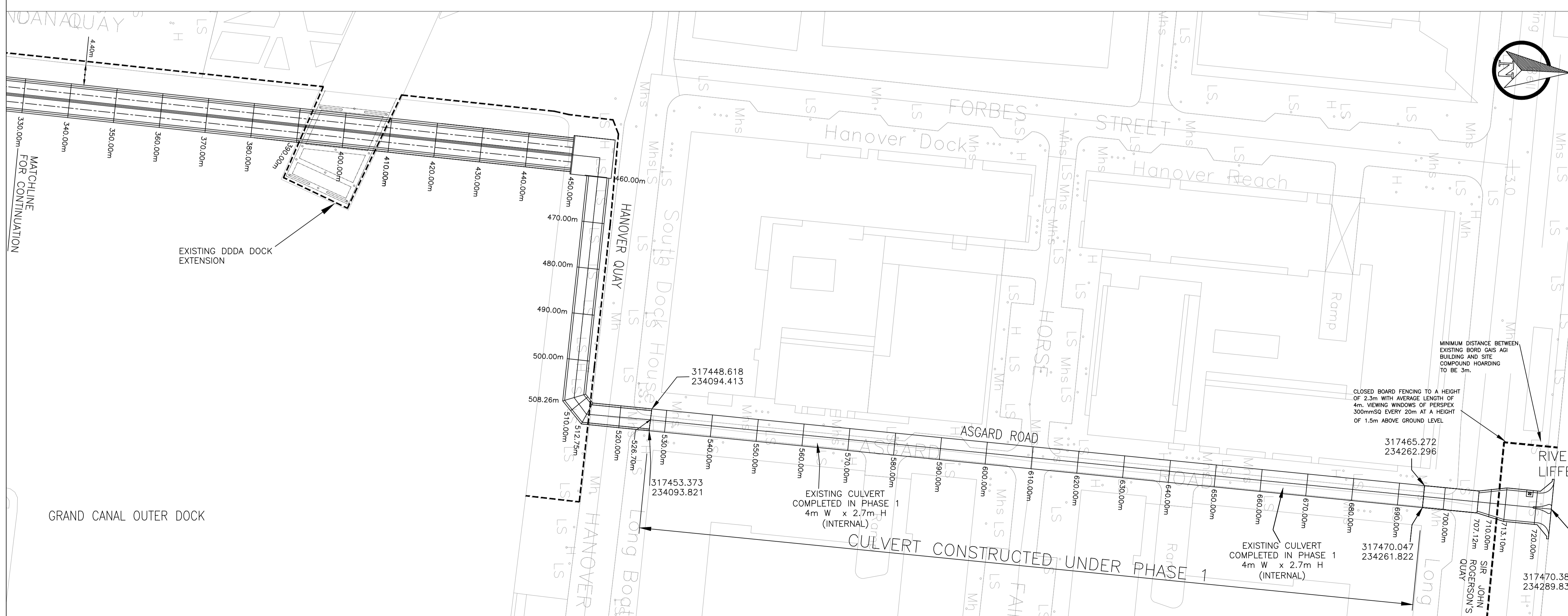
PLAN OF PIPELINE (CHAINAGE 340.00m TO RIVER LIFFEY)
