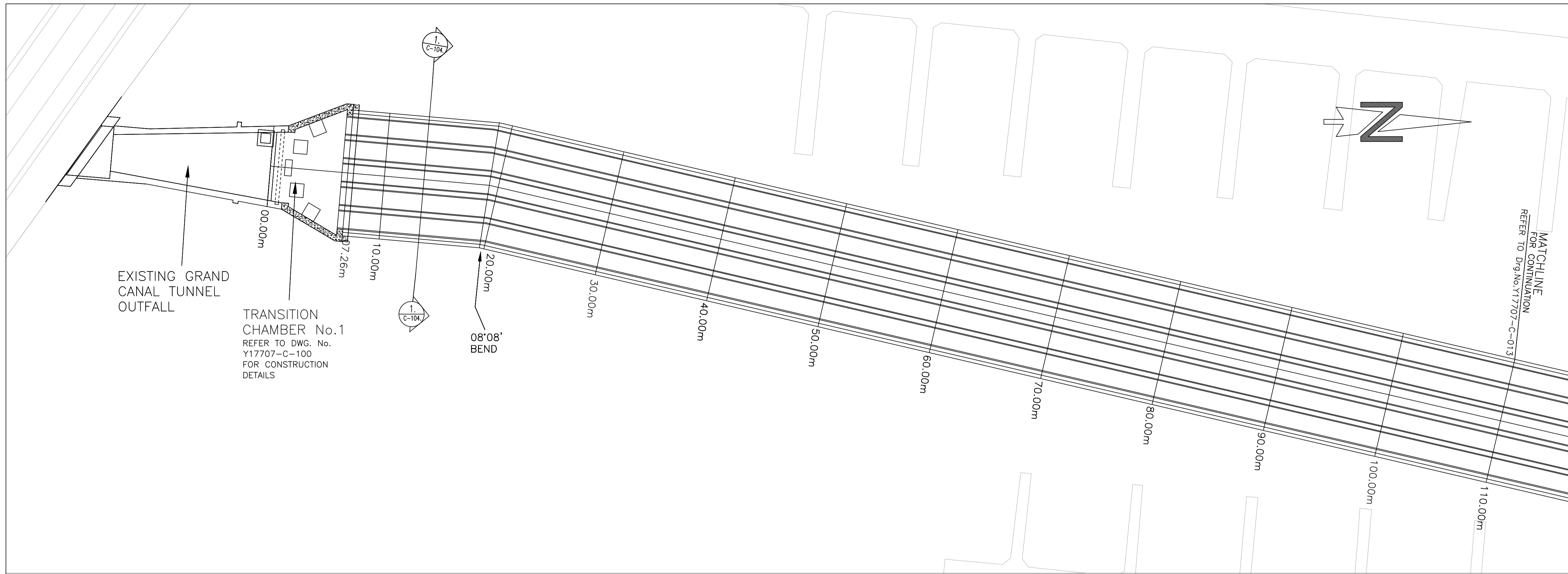
PLAN OF PIPELINE (CHAINAGE 0.00m TO 110.00m) SCALE : 1:200
