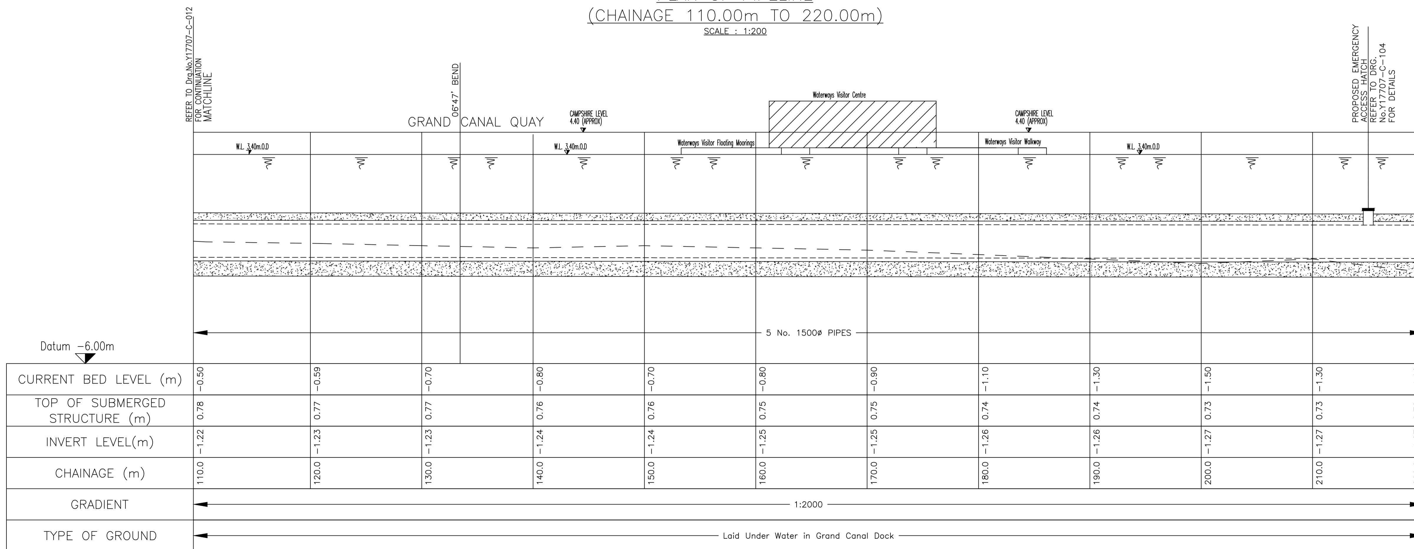
LONGITUDINAL SECTION THROUGH PIPELINE (CHAINAGE 110m TO 220m) SCALE : HOR=1:200 VERT.=1:100
