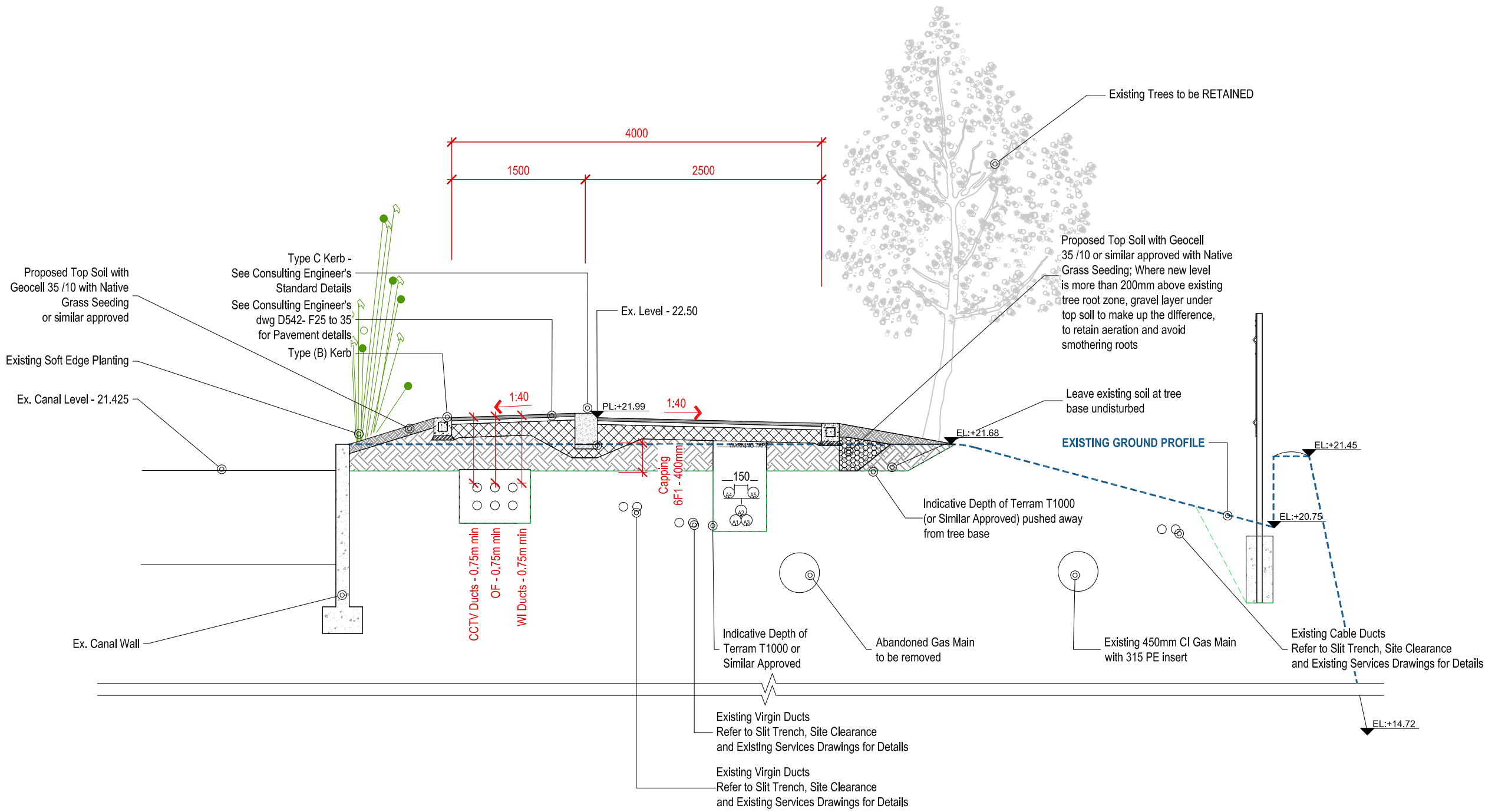
C-C TYPICAL CROSS SECTION C-C LINEAR PARK DR-401 PLAN B 470 Scale 1:50
