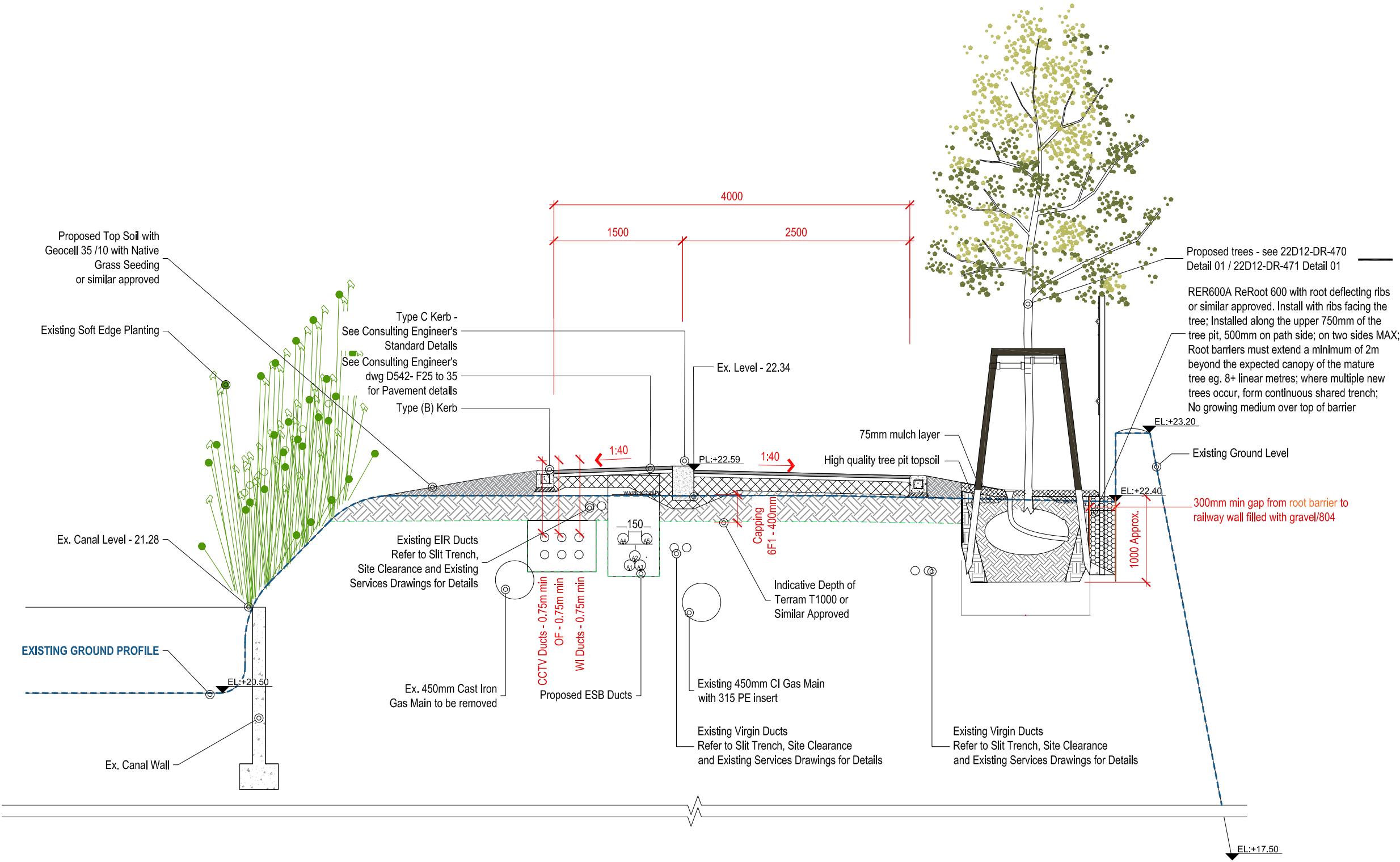
A-A TYPICAL CROSS SECTION A-A LINEAR PARK DR-401 PLAN A 470 Scale 1:50
