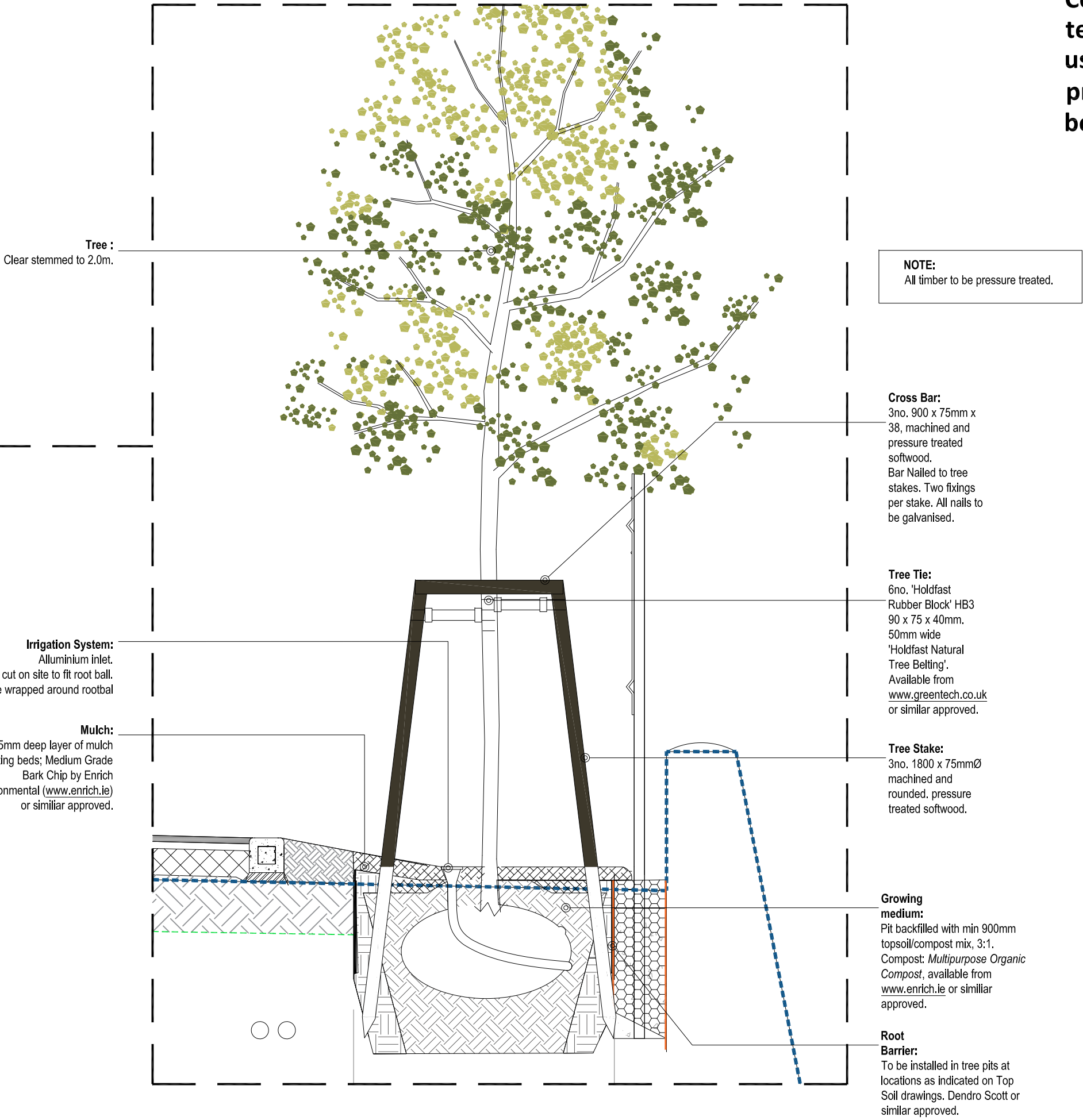
01 TYPICAL SEMI-MATURE AND HEAVY STANDARD TREE PLANTING DETAIL 470 Scale 1:25
