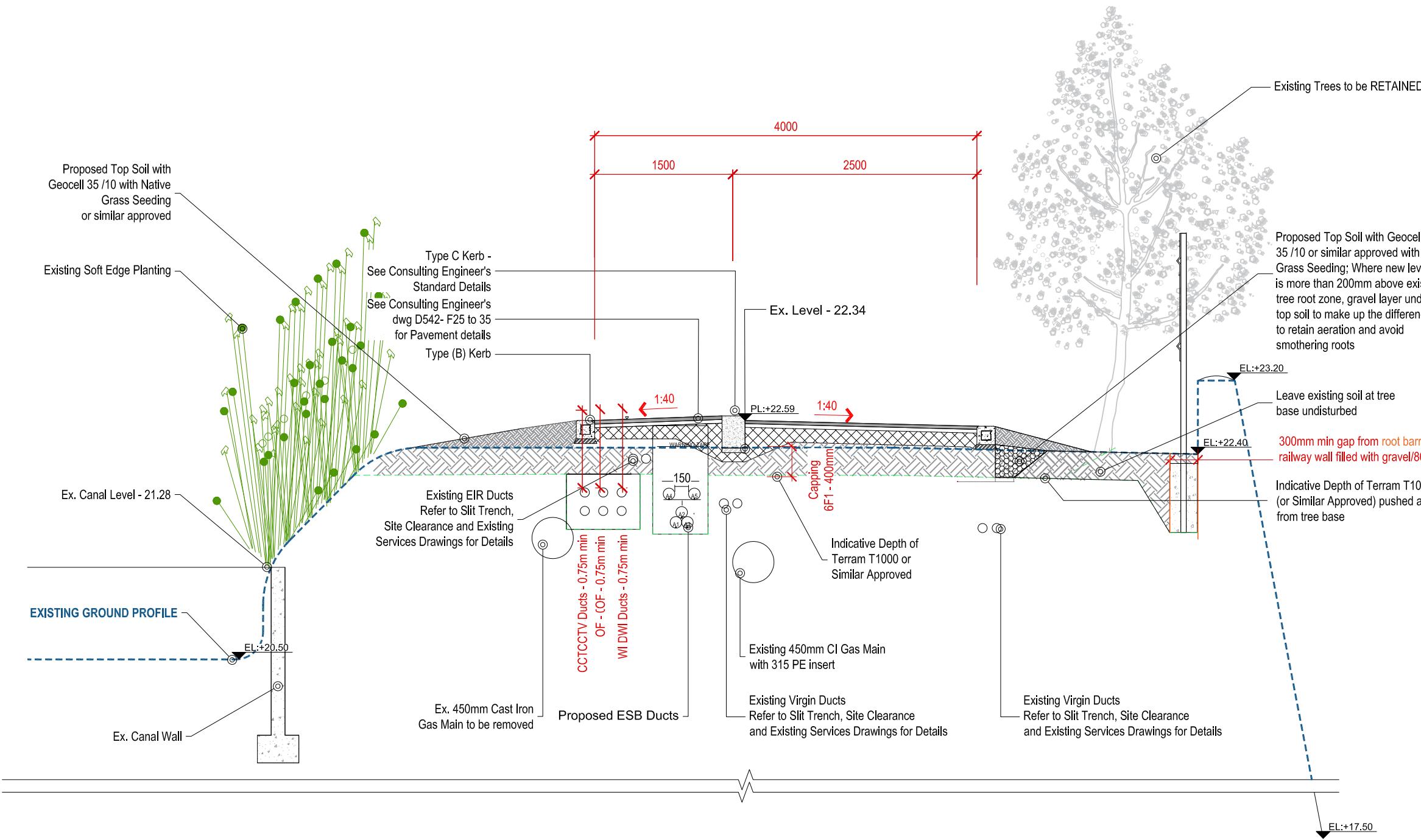
B-B TYPICAL CROSS SECTION B-B LINEAR PARK DR-401 PLAN A 470 Scale 1:50
