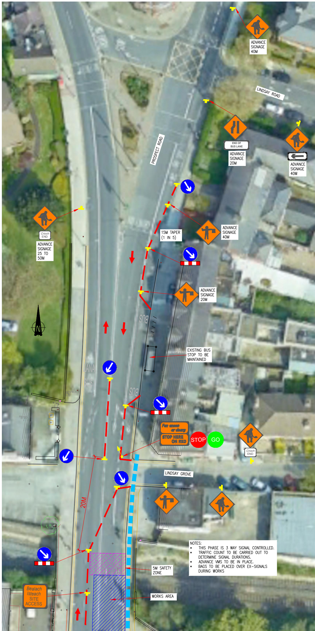
WORKS AREA AT PHILSBOROUGH ROAD JUNCTION - SURFACING STAGE 1
