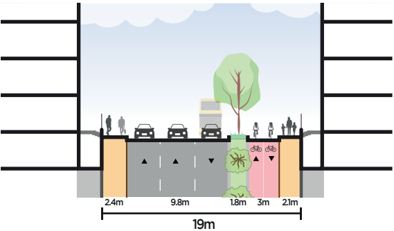
Figure 9.7.1 - Section Gardiner Street Proposed
