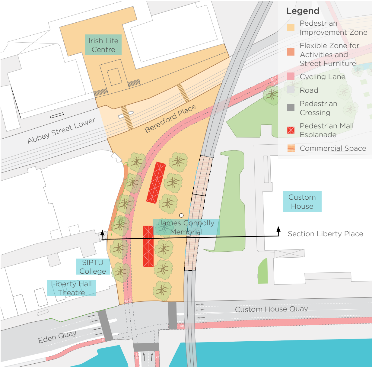
Figure 9.5.2 – Plan Liberty Place Proposed
