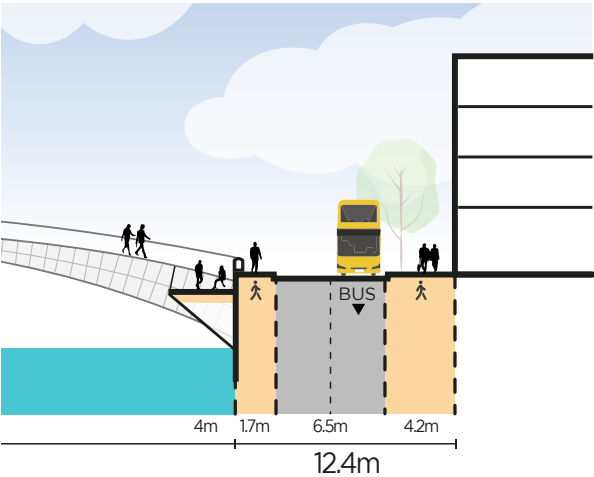
Figure 9.4.1 – Section South Quays Proposed
