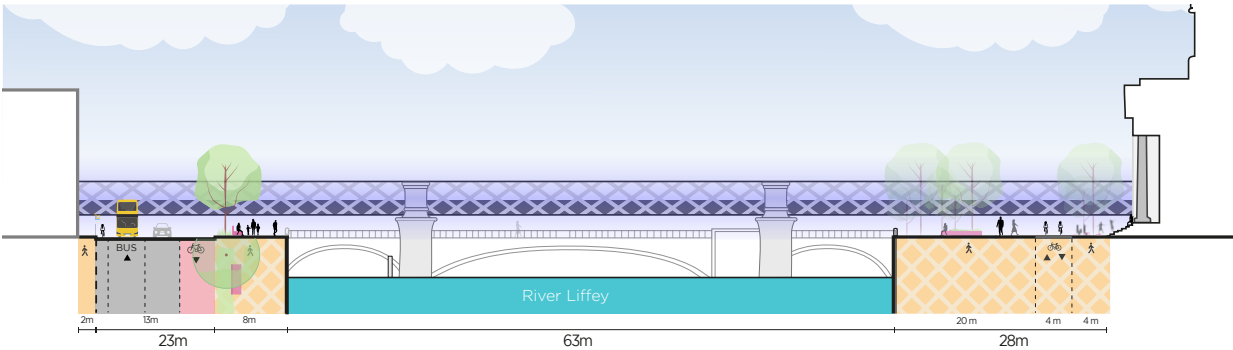
Figure 9.6.2 – Section Custom House Quay Proposed
