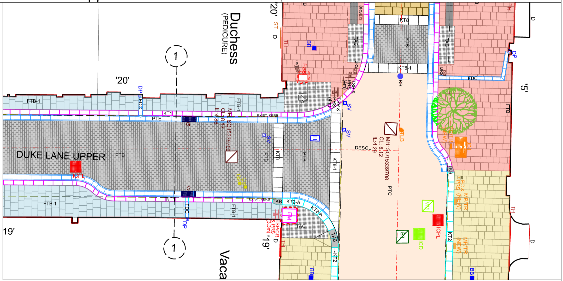
PLAN - DUKE LANE UPPER. (Contd.)
