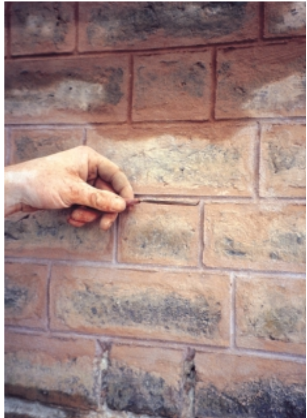
Brick pointing detail
