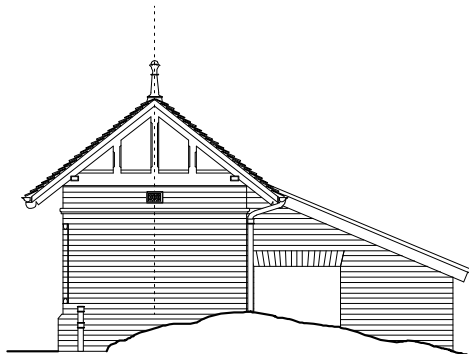
west elevation
